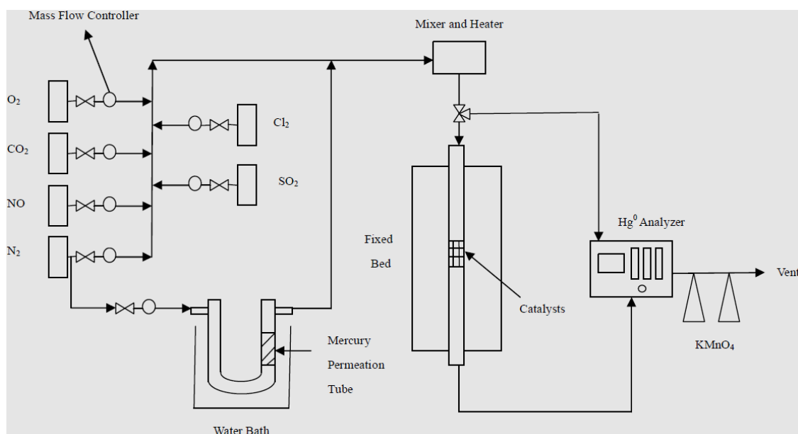
Fig. 8: Schematic diagram of fixed-bed reactor system.
