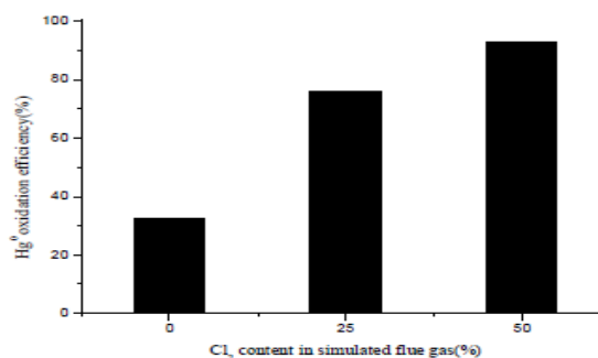
Fig. 6: Effect of \text{Cl}_2 on \text{Hg}^0 oxidation.
