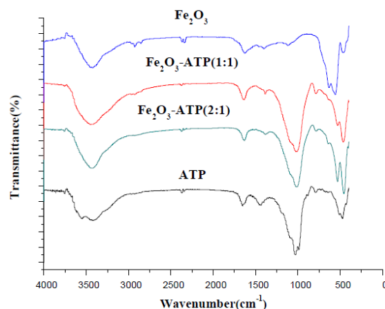
Fig. 3: FT-IR spectra of ATP(calcined at 500°C), \text{Fe}_2\text{O}_3 , \text{Fe}_2\text{O}_3 -ATP(1:1) and \text{Fe}_2\text{O}_3 -ATP(2:1).
