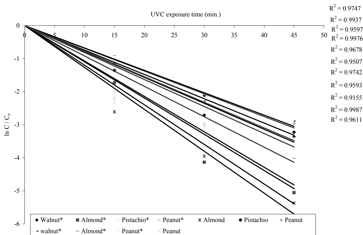
Fig. 3: Degradation kinetics for AFB 1 following UVC exposure in nuts at different moisture levels.
