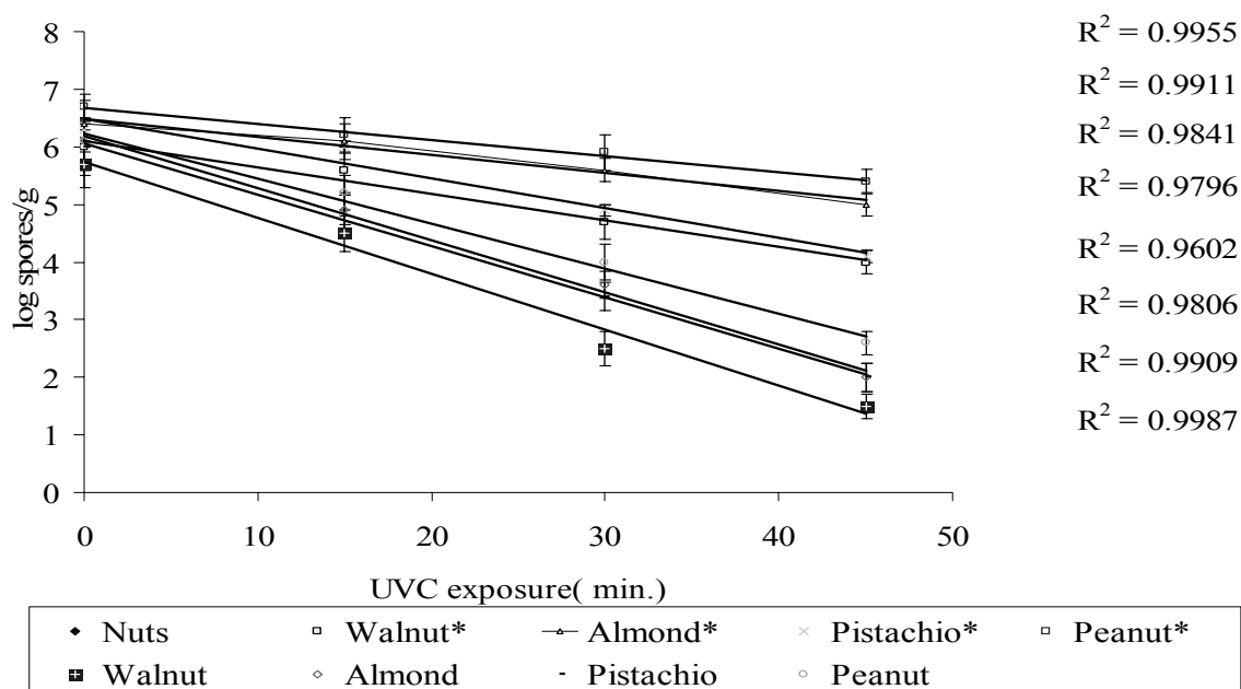
Fig. 1: Effect of UVC exposure on fungal count in twelve week stored ground and tree nuts.
