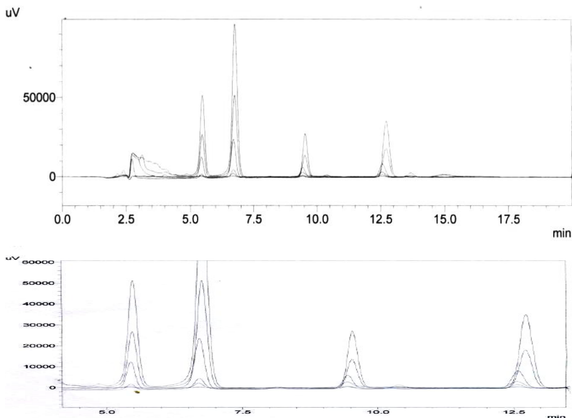
Fig. 2: Chromatographs of standard calibration solutions showing excellent repeatability and reproducibility for AFG 1 , AFB 1 , AFG 2 and AFB 2 respectively.
