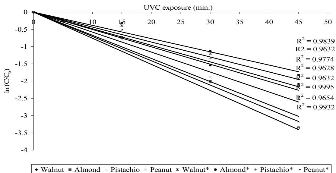
Fig. 3: Degradation kinetics for AFB 1 following UVC exposure in nuts at different moisture levels.
