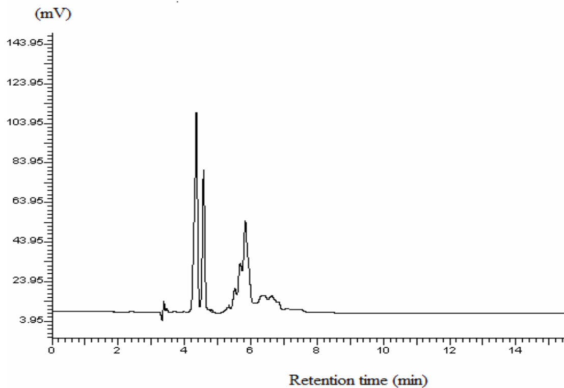
Fig. 7: Chromatogram for 10 µg g -1 fenoxaprop- p -ethyl fortified soil sample using reverse-phase HPLC.
