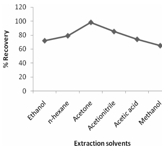
Fig. 1: Investigation for suitable solvent for extraction of fenoxaprop-p-ethyl.
