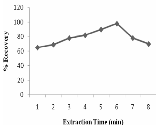
Fig.4: Effect of microwave extraction time on % recovery of fenoxaprop-p-ethyl.
