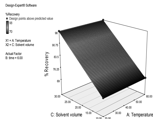
Fig. 5: Response surface plot for % recovery of fenoxaprop-p-ethyl.
