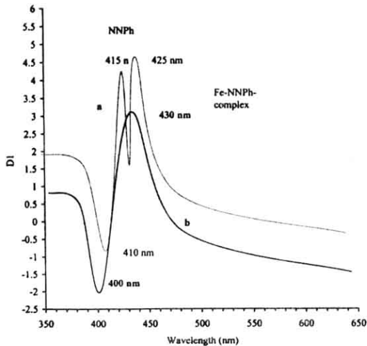
Fig. 1: First derivative spectra of (a) 1-nitroso-2-naphthol (b) iron (III)-1-nitroso-2-naphthol complex in 5% Tween 40 at pH 1.
