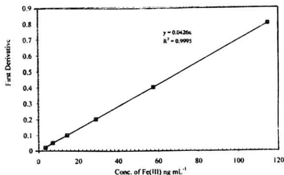
Fig. 5: Calibration graph of Fe(III)-1-nitroso-2-naphthol complex in 5% Tween 40 at pH 1 at ( \lambda_{\text{max}} 430 nm and 400 nm) in first derivative mode spectroscopy.
