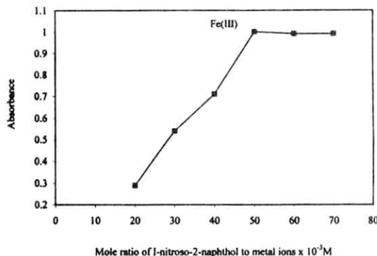
Fig. 3: Effect of amounts of 1-nitroso-2-naphthol on the absorbance of Fe(III).
