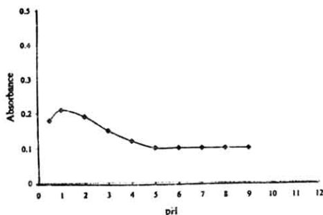
Fig. 4: Effect of pH on the absorbance of metal-1-nitroso-2-naphthol complex.
