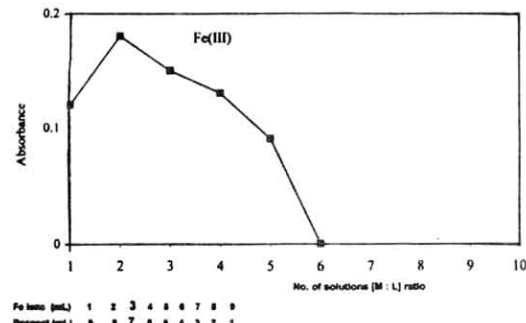
Fig. 2: Job's plot of metal: ligand ratio.
