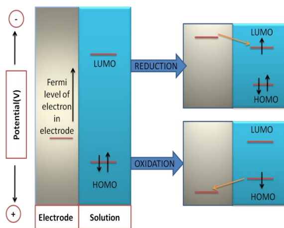
Fig. 1: Illustration of the charge transfer energetic across the electrode/solution interface.
