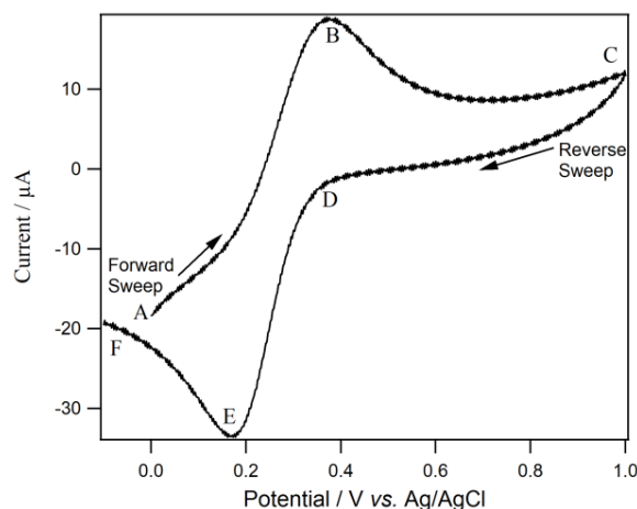
Fig. 3: CV of 5 mM \text{K}_3[\text{Fe}(\text{CN})_6] solution at 3 mm diameter GC vs. Ag/AgCl at 50 \text{ mV s}^{-1} .
