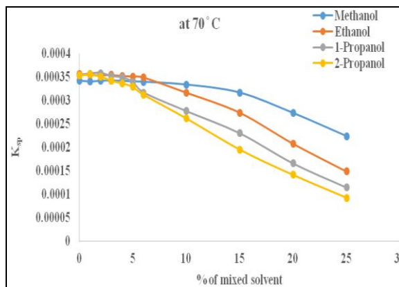
Fig. 4: Effect of added solvents on the K_{sp} of Strontium hydroxide at 20 °C and 70 °C.
