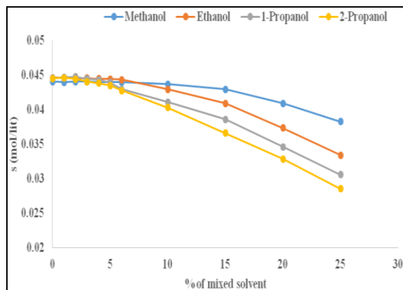
Fig. 3: Effect of added solvents on the molar solubility ( s ) of Strontium hydroxide at 20°C and 70°C.
