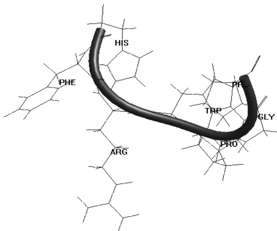
Fig. 1: Spatial structure of amino acids in low-energy conformations: a) R 13 B 1 B 3122 B 11 BPR, b) B 21 B 1 B 3322 B 11 RPR, c) B 21 R 3 B 3322 B 11 BLR.
