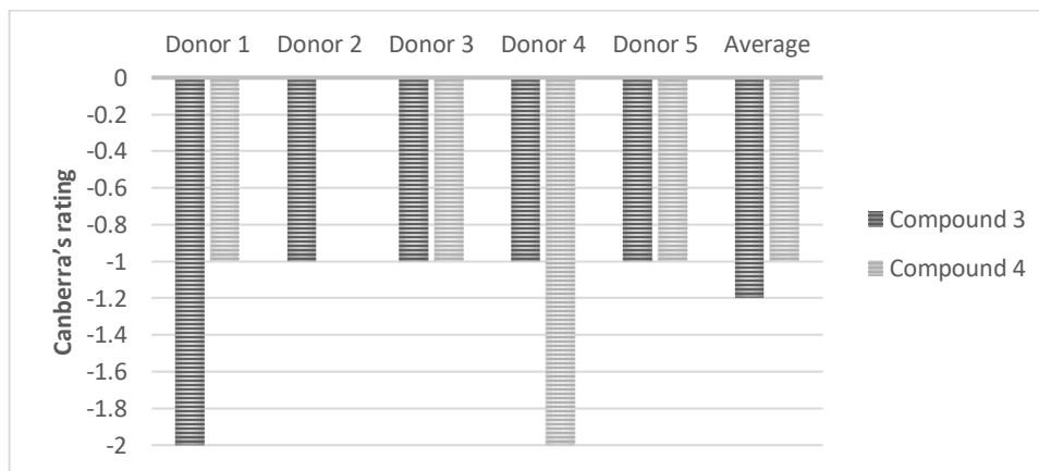
Fig. 9: Development quality (Canberra's rating) for phenothiazines 3 and 4.
