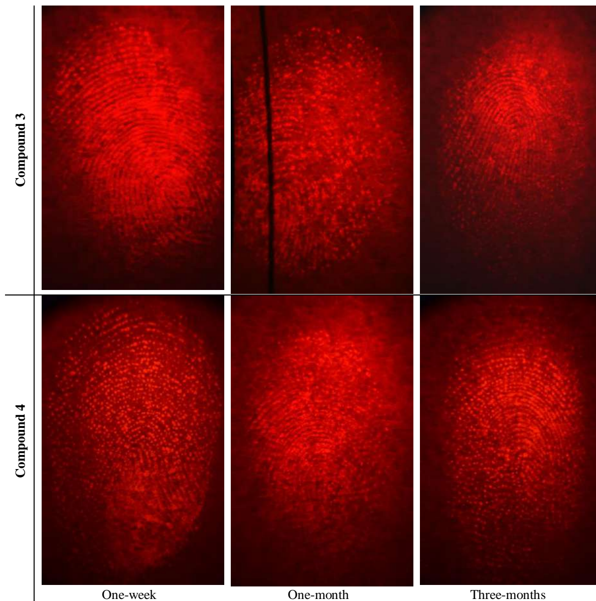
Fig. 6: Aged latent fingerprints developed with phenothiazines 3 and 4 .
