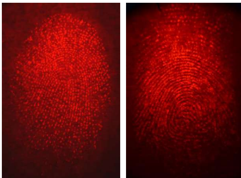
Fig. 4: Latent fingerprints (one-day) developed with phenothiazines 3 (a) and 4 (b).
