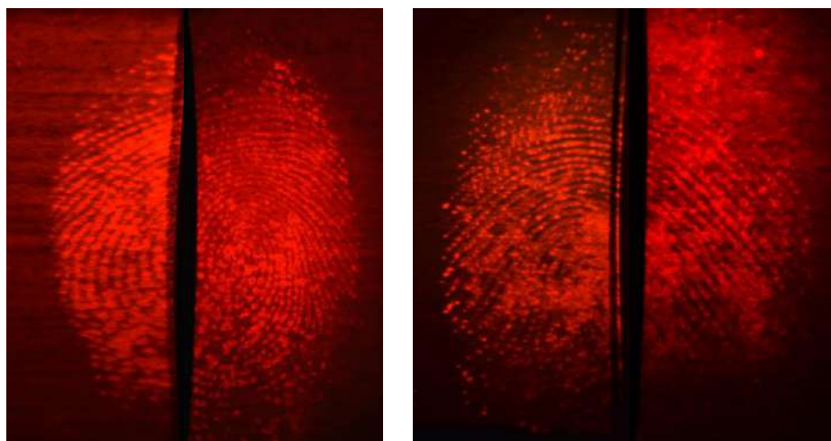
Fig. 8: Comparison between development of latent fingerprints (one-day) with DFO (left) and phenothiazines 3 (a) and 4 (b) (right).
