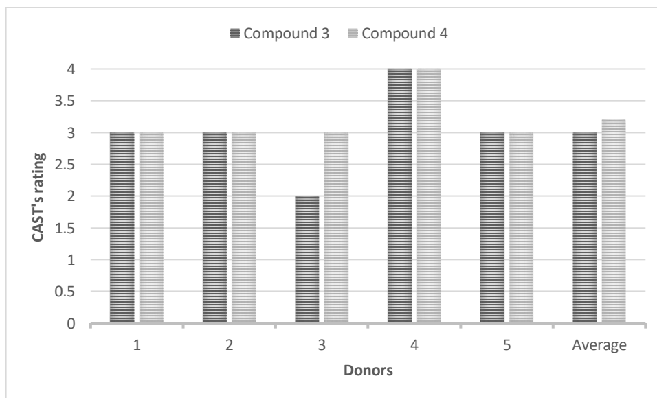
Fig. 5: Development quality (CAST's rating) for phenothiazines 3 and 4.
