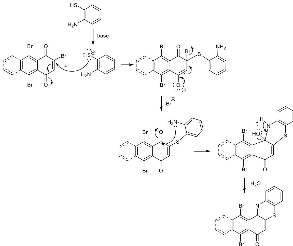
Fig. 3: The reaction mechanism for the formation of the 3 and 4 .
