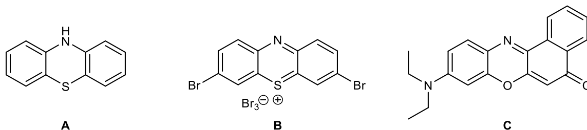
Fig. 1: Chemical structures of phenothiazine (A), 3,7-dibromophenothiazin-5-ium (B), and Nile red (C).
