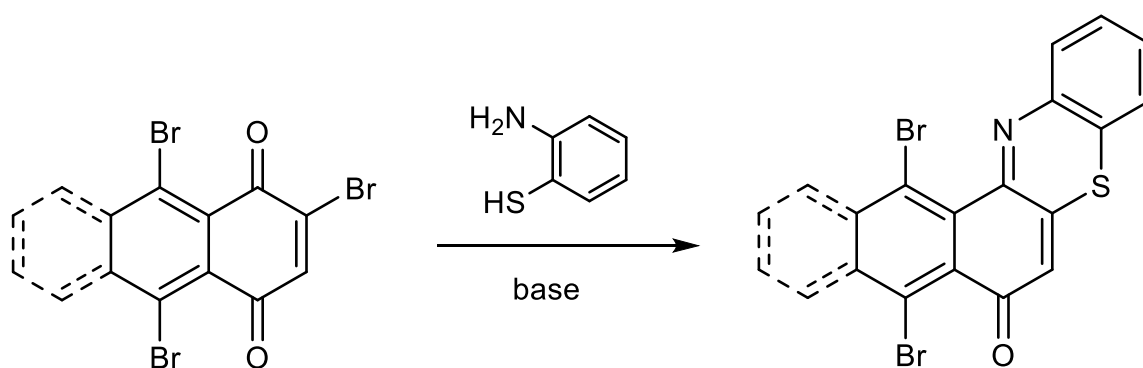
Fig. 2: Synthesis of phenothiazines 3 and 4 .
