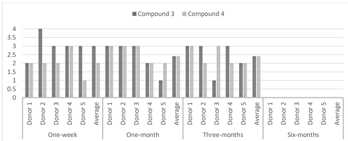
Fig. 7: Development quality (CAST's rating) for aged latent fingerprints developed with phenothiazines 3 and 4.
