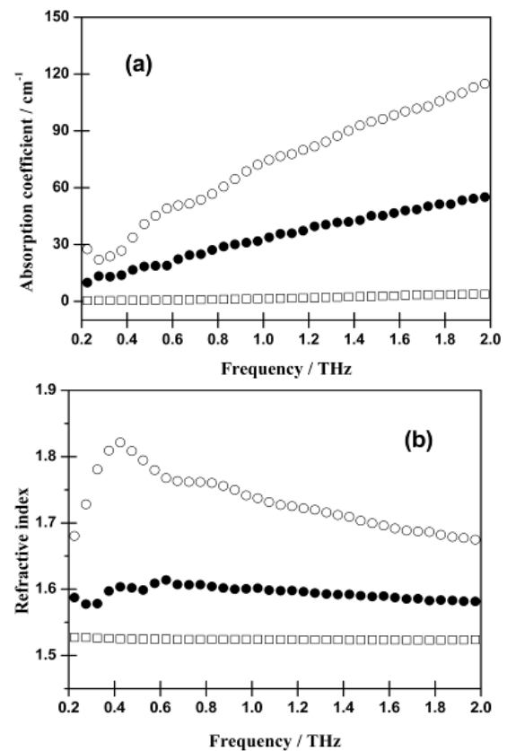
Fig. 2: The frequency dependence of \alpha (a) and n (b) for HDPE( \square ) and composites filled with 2.20% thin-MWNT( \bullet ) and thick-MWNT( \circ ), respectively.
