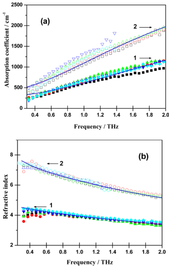
Fig. 3: \alpha (a) and n (b) obtained by MG fitting as a function of frequencies for thin-MWNT (1) and thick-MWNT (2), respectively. \blacksquare/\square : 1.10%, \bullet/\circ : 2.20%, \blacktriangle/\triangle : 3.37%, \blacktriangledown/\triangledown : 4.48%, \blacklozenge/\lozenge : 5.72%. The solid lines are fittings with Drude-Lorentz model.
