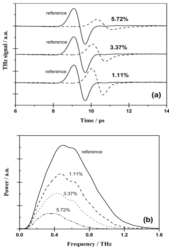
Fig. 1: Time-domain wave forms (a) and frequency-domain spectra (b) for the reference and composites filled with thin MWNTs at different concentration.
