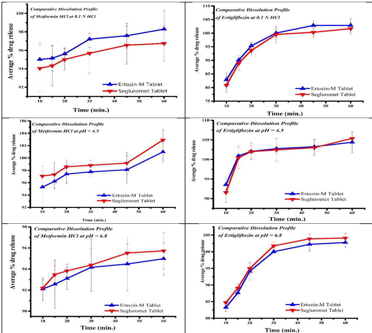
Fig. 6: Comparative dissolution profiles of MET and ERT at different pH.
