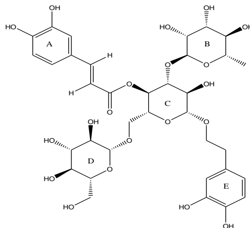
Fig. 1: The chemical structure of Echinacoside.
