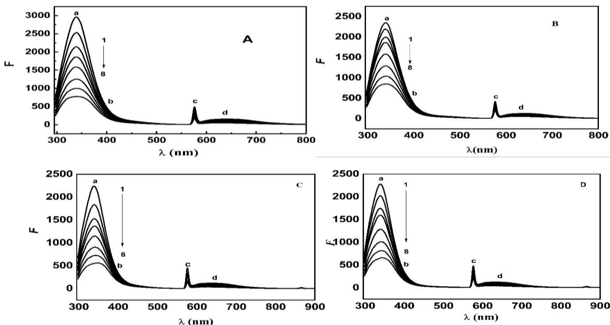
Fig. 5: Fluorescence quenching spectra of HSA interacting with ECH/VER c_{(\text{HSA})}=1.0\times10^{-5}\text{mol L}^{-1} , c_{(\text{VER/ECH})}/10^{-5}\text{mol L}^{-1} , 1 to 8: 0.0, 0.4, 0.8, 1.0, 1.6, 2.4, 3.2, 4.0. A: VER-HSA 25°C; B: VER-HSA 37°C; C: ECH-HSA 25°C; D: ECH-HSA 37 °C
